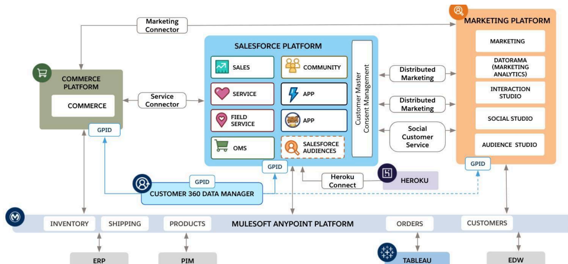
Figure 1: Architecture and data flow of the customer support & service automation
